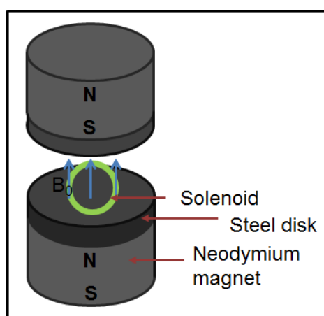
Fig. 5. Helmholtz sensor design. Magnets are separated by 20 mm, in the gap there is a homogeneous magnetic field in which the solenoid coil is installed. Steel disks are placed on each magnet to reduce the field gradient.
