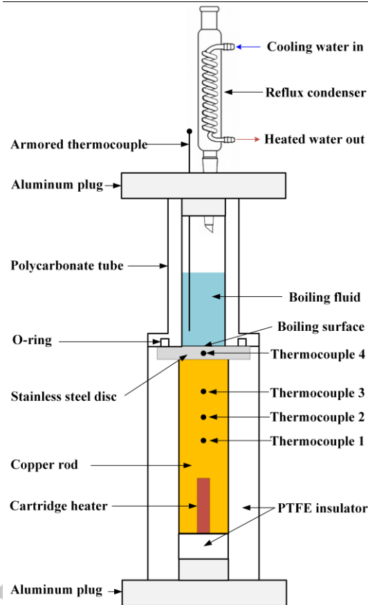
Fig 1 Schematic of nucleate pool boiling experimental facility
