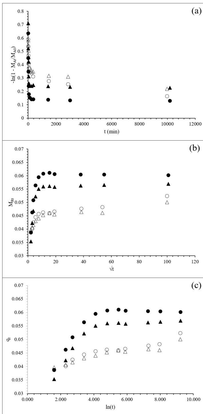
Figure 7. Kinetic fitting of cobalt and nickel uptake by EBP-Si and S950 using (a) film diffusion model, (b) pore diffusion model and (c) Elovich model at pH 2.0 and 4.3 respectively. Circles = Co 2+ and triangles = Ni 2+ , open symbols = EBP-Si and closed symbols = S950.
