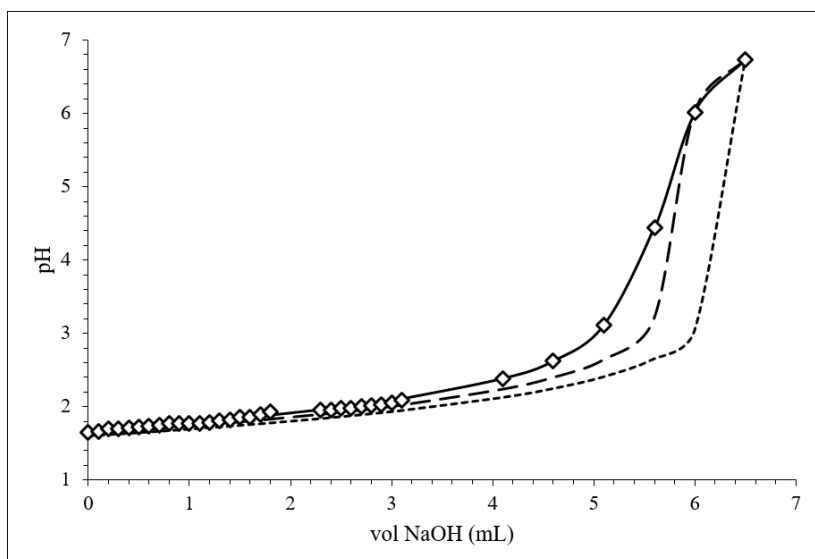
Figure 2. Potentiometric titration of EBP-Si at 21 °C and I = 1M (NaCl). Diamonds = experimental data points. PSEQUAD program fits are shown by black lines: solid line = 3 pK a fit, dashed line = 2 pK a fit, dotted line = 1 pK a fit.
