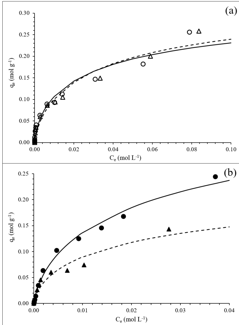
Figure 6. Isotherms for cobalt and nickel uptake on (a) EBP-Si at pH 2.0 and (b) S950 at pH 4.3, 21 °C and 24 hr contact fitting using D-R isotherm model. Circles = \text{Co}^{2+} and triangles = \text{Ni}^{2+} , black solid line = \text{Co}^{2+} D-R fit, black dashed line = \text{Ni}^{2+} D-R fit.
