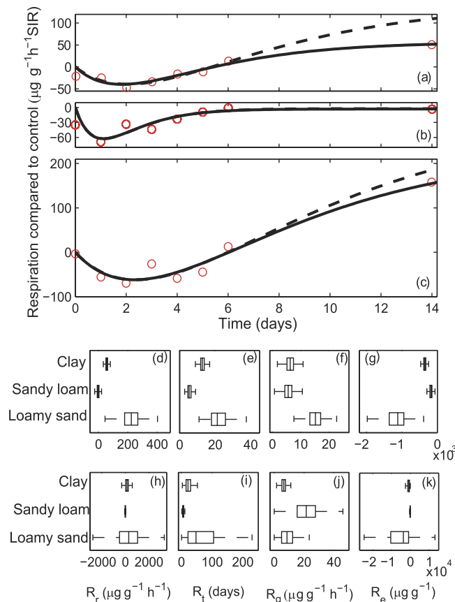
Figure 6. Change in substrate induced respiration of (a) clay, (b) sandy loam and (c) loamy sand soil samples after the addition of 1000 \text{ mg triclosan kg}^{-1} dry mass showing data (circles) and the modelled response fitted either with (solid lines) or without (dashed lines) the last data point. Note that the two modelled responses are almost identical in the sandy loam. Measurements are the difference in SIR (glucose substrate) between a perturbed and a control sample, with each measurement made destructively. The resilience characteristics (Table 1) identified using the model fitted to all the data (d–g) and the model fitted without the last data point (h–k). Boxplots show the median (central mark), interquartile range (box) and range (whiskers) with outliers excluded.
