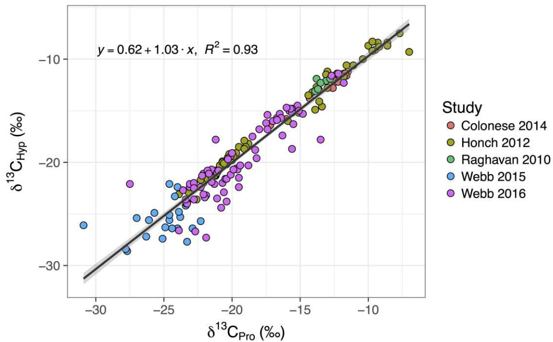
Figure 2. Comparison of published collagen and dentin proline and hydroxyproline \delta^{13}C values from archaeological materials shows that there are only minor offsets between these amino acids ( y = 0.62 + 1.03x , adjusted R^2=0.9252 , F(1,184)=2290 , P<0.001 ). The data were obtained from five studies that used LC/IRMS [68-72]. The solid lines depict the linear correlations, and the shaded areas depict 95% confidence intervals.
