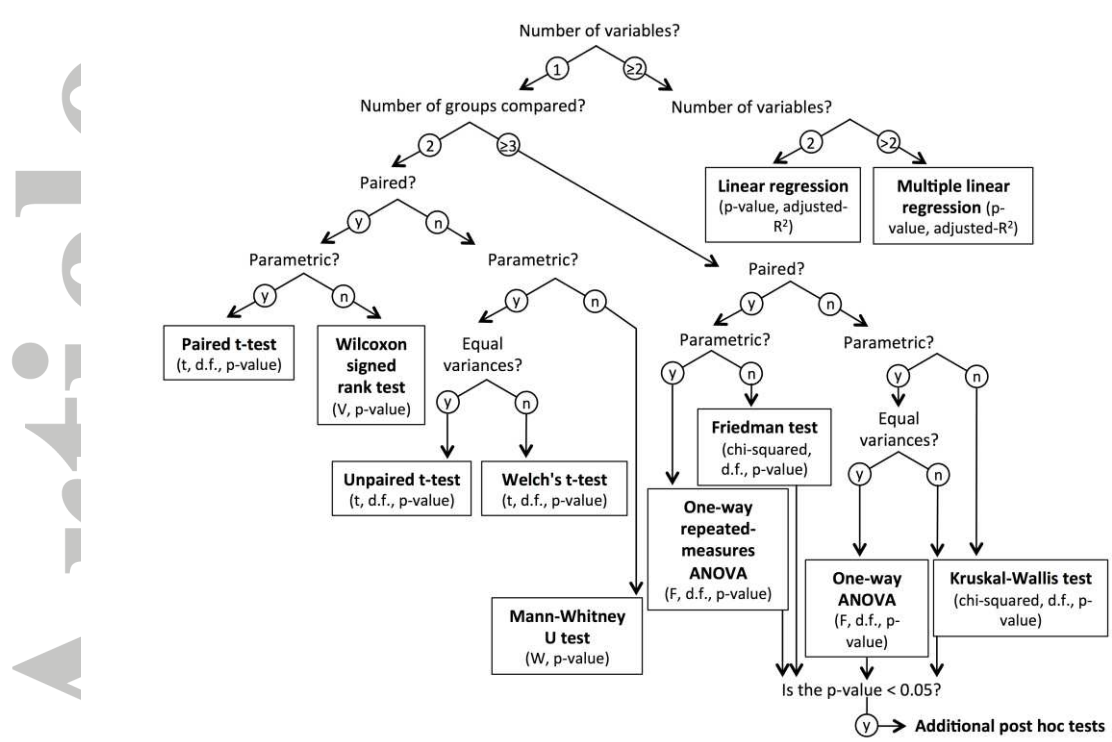
Figure 7. Comparison of different, commonly-used statistical analyses potentially useful for evaluating \delta value differences between groups in archaeological datasets (based on McCrum-Gardner [75] and Marusteri and Bacarea [76]).
