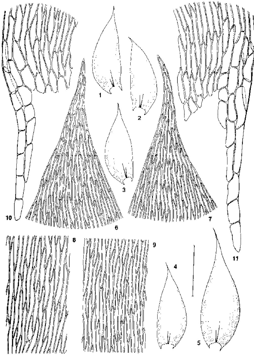
Fig. 1: Plagiothecium lucidum (Hook. f. & Wils.) Paris. 1–5: Leaves. 6–7: Leaf apices. 8–9: Mid-leaf cells. 10–11: Alar cells (1–3, 7, 9, 11 drawn from Standley & Valerio 43764, isotype of Isopterygium integrifolium , FH; from Miehe 3135, KRAM; 4–6, 8, 10). Scale bar: 1 mm (1–5) and 100 \mu m (6–11).
