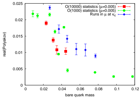
Figure 7: Comparison of runs for different (\kappa, \mu) pairs at \beta = 3.9 mapped to the bare quark mass.
