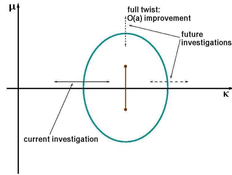
Figure 8: Current and planned investigations in the context of the expected phase structure.
