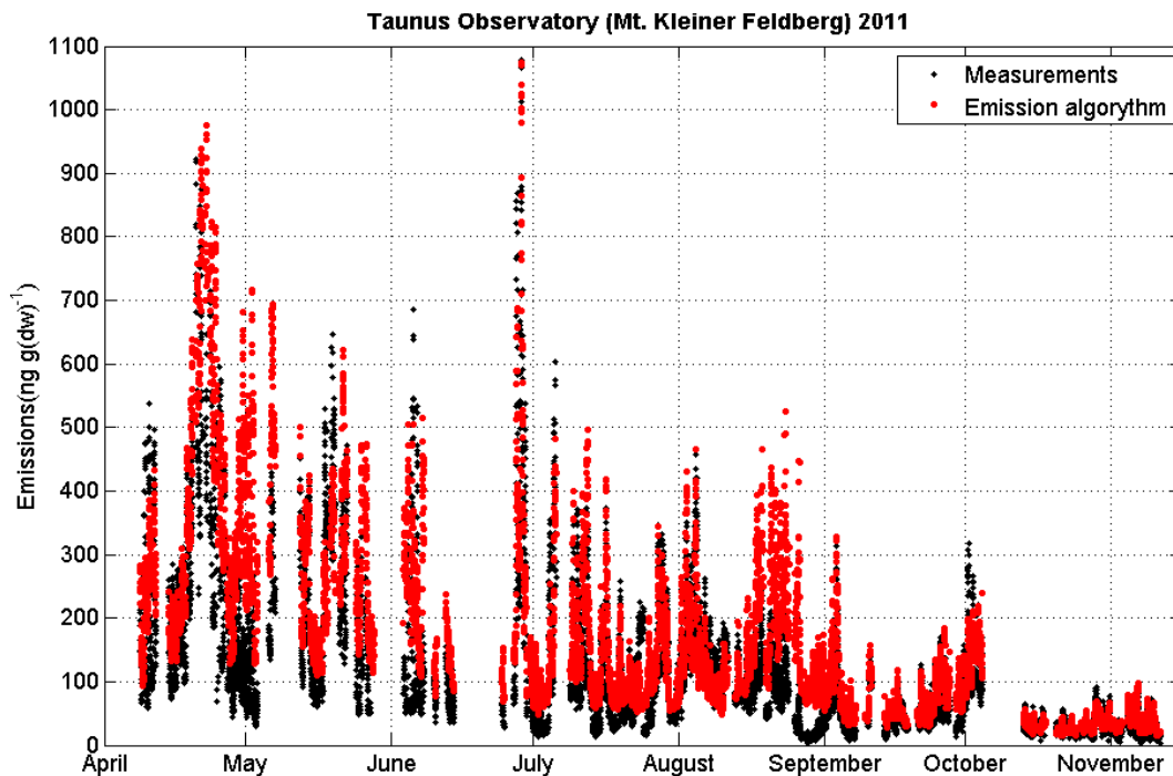
Fig. 8. Temporal pattern of the measurements compared with the new emission algorithm.
