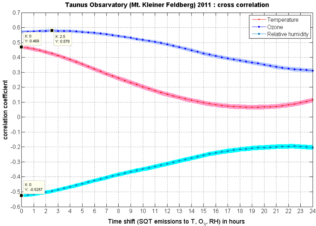
Fig. 3. Cross-correlation of SQT emission and temperature (red), ozone (blue) and relative humidity (cyan), with a time shift between the emissions and the individual stress factors.
