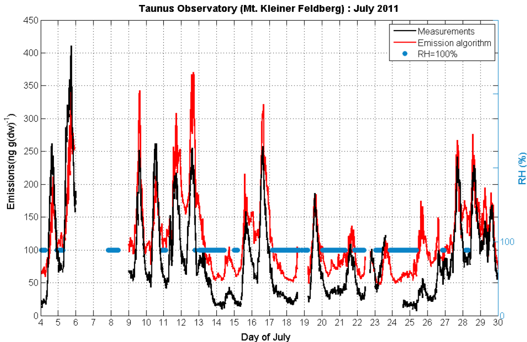
Fig. 9. Example of how RH can influence SQT emission rates derived from Eq. (5). In case of RH = 100 %, the algorithm fails, since the thin water layer created above the needle surface acts in protective way for the involved stresses.
