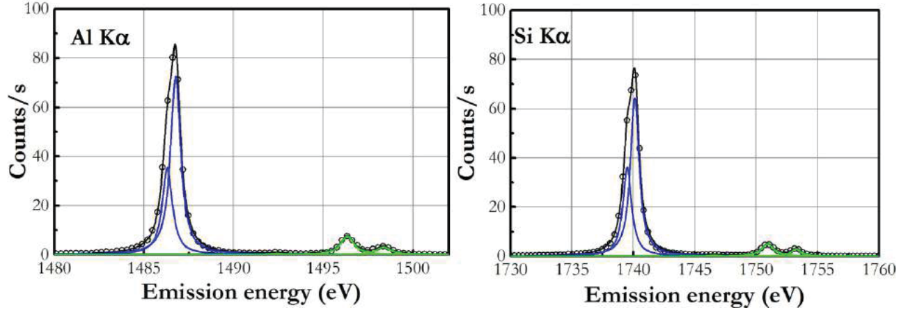
FIG. S1. Reference K\alpha x-ray spectra of elemental Al and Si. For the fit Lorentzian profiles were used. The FWHM experimental energy resolution was derived from the fitted Lorentzian widths by subtracting the natural lifetime broadening of 0.41 eV for Al, and 0.48 eV for Si. The widths were adopted from the recommended values of Campbell and Papp (reference [33] in the manuscript). FWHM experimental energy resolution of 0.27 eV at 1.487 keV, and 0.38 keV at 1.740 keV was obtained. The lines occurring around 1497 eV and 1752 eV correspond to the K\alpha_{1,2}L_1 satellites of Al and Si, respectively.
