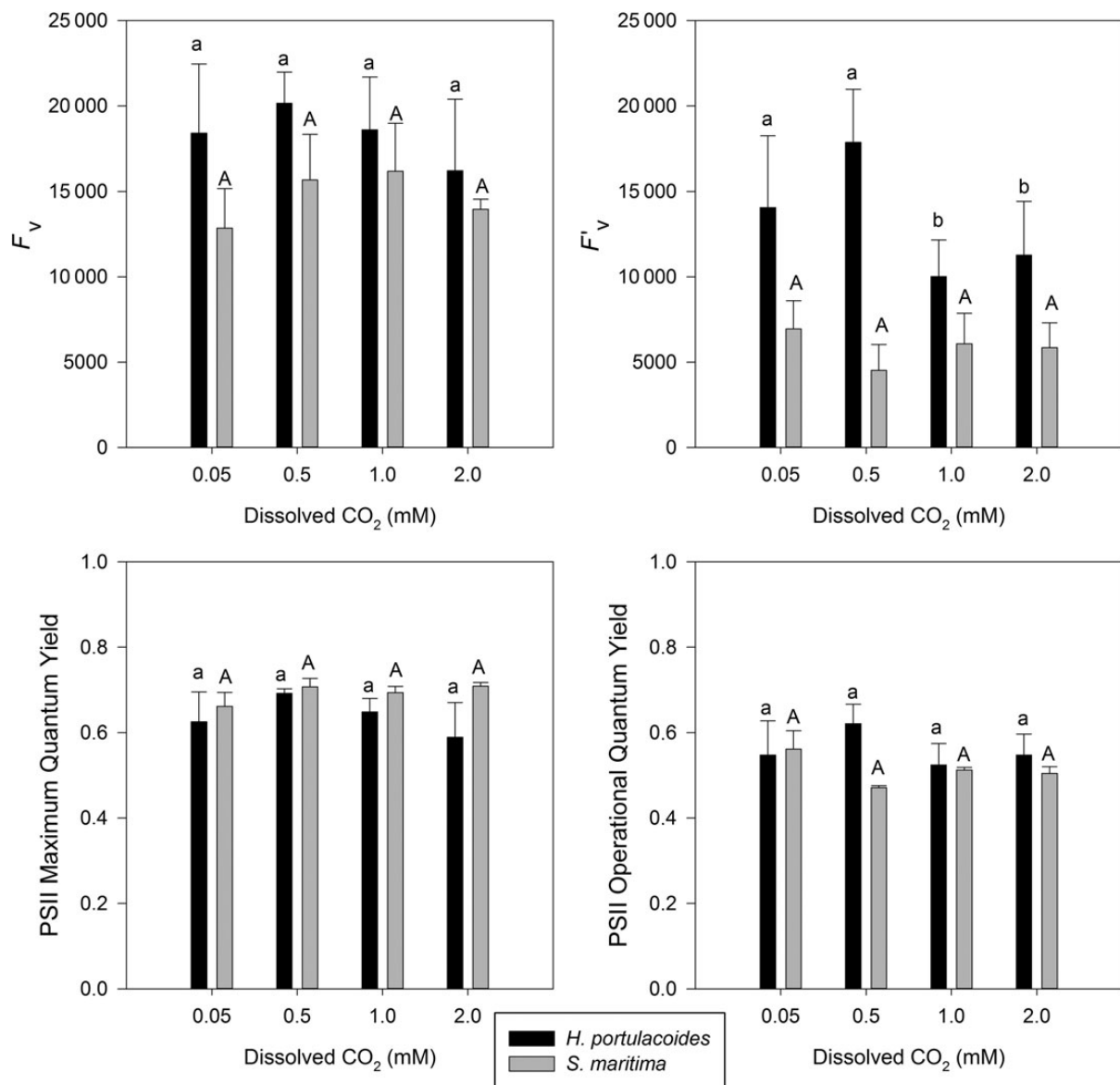
Figure 2. Photosystem II variable fluorescence and quantum efficiencies (operational and maximum) by the two tested species under light and dark conditions, at different levels of dissolved CO 2 (average \pm standard deviation, n = 9 ). Letters indicate significant differences among CO 2 treatments at P < 0.05 .
