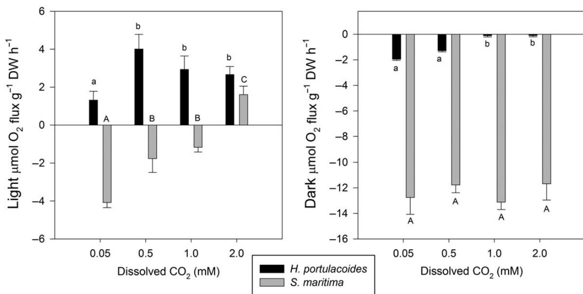
Figure 1. Oxygen production and consumption by the two tested species under light and dark conditions, at different levels of dissolved CO 2 (average \pm standard deviation, n = 9 . Letters indicate significant differences among CO 2 treatments at P < 0.05 ).
