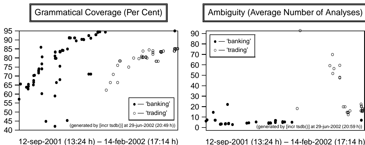
Figure 2: Evolution of grammatical coverage and average ambiguity (number of readings per test item) over a five-month period; ‘banking’ and ‘trading’ are two data sets (of some 700 and 400 sentences, respectively) of domain data.
