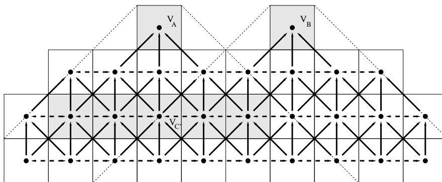
Fig. 7 The mixed acyclic graph generated by boxes of equal size covering of the 1+1 dimensional Minkowski spacetime.
