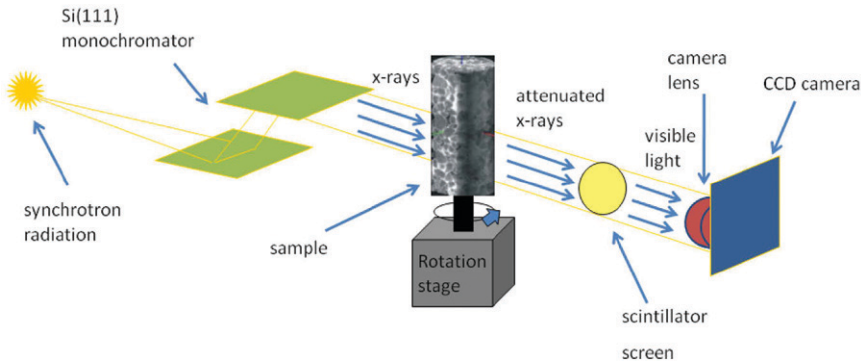
Fig. 1–3. Typical synchrotron tomography beam-line setup.
