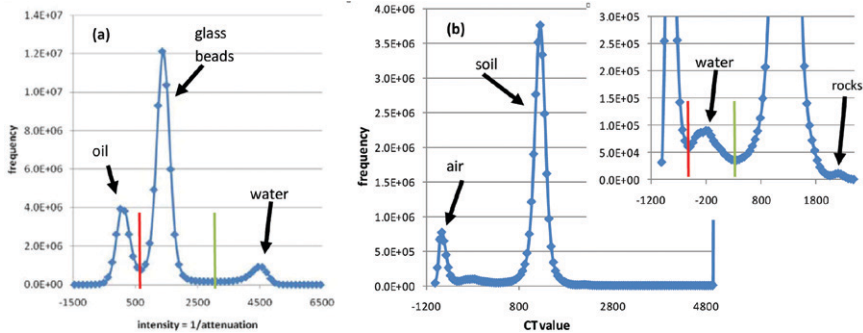
Fig. 1–4. (a) Synchrotron-based image of a partially saturated glass bead pack imaged at 10.8\ \mu\text{m} . Using the new optics and lutetium–aluminum–garnet scintillator the different phases (oil, water, beads) are easily separated. (b) Typical medical computed-tomography (CT)-based histogram for a partially saturated clayey till soil column imaged at \sim 600\ \mu\text{m} . Four different phases (air, water, soil, rocks) can be identified based on the histogram.
