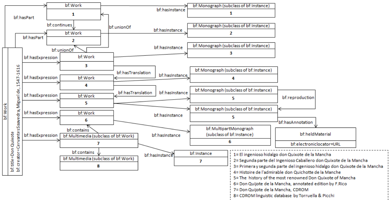
Figure 3: BIBFRAME representation
