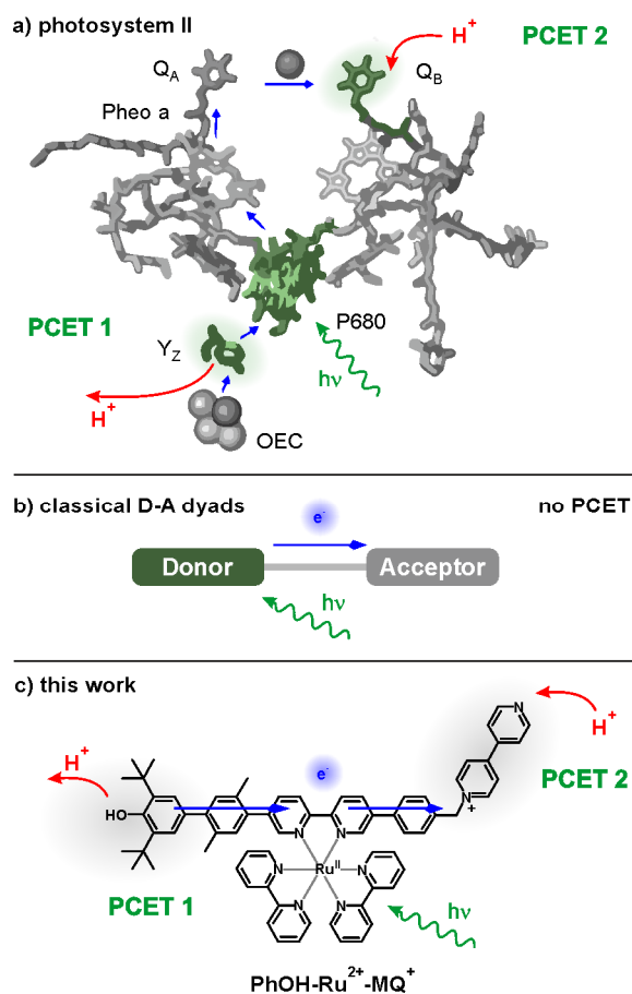
Figure 1. (a) Primary and secondary electron transfer events (blue arrows) in photosystem II after excitation of P680 (green central part). PCET occurs at tyrosine Z (green, lower left) and at plastoquinone B (green, upper right). 3 (b) Generic donor-acceptor compound exhibiting simple electron-hole separation. (c) Investigated triad comprised of a phenol donor (PhOH) resembling tyrosine Z (PCET 1), a Ru(II) sensitizer mimicking the function of P680, and a monoquat acceptor (MQ + ) playing the role of plastoquinone B with regard to uptake of one electron and one proton (PCET 2).
