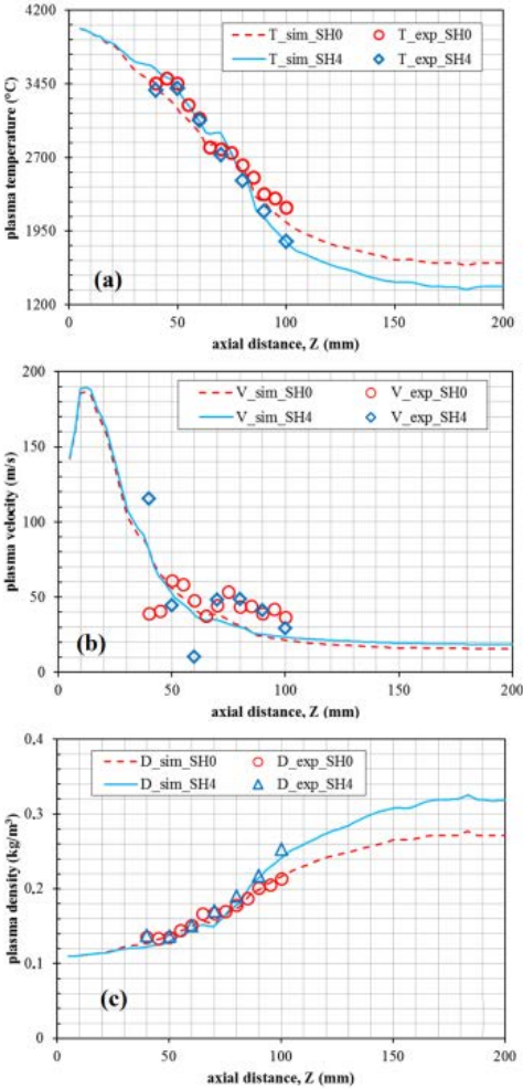
Fig. 7 measured and simulated characteristics of the plasma jet: temperature (a), velocity (b)
