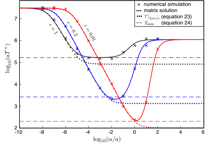
FIG. 3. The mean extinction time as a function of \alpha for three different choices of \epsilon = 1 (black), 0.2 (blue), 0.01 (red), all possessing equivalent \alpha \rightarrow \infty extinction times ( \bar{\tau} ). Four metrics are plotted: Crosses denote the mean extinction time computed using direct simulations, solid lines were computed using the matrix equation (8), dotted lines depict our heuristically derived approximation in the regime where \alpha \ll a [Eq. (23)], and the dashed line denotes the expected minimum extinction time [Eq. (24)] using the arguments in the text. As expected, red and blue graphs turn off into the minimum at 1/\alpha roughly corresponding to the extinction time in the bad state \log_{10}(\alpha/a) = -2.4 for A = 1.6 and \log_{10}(\alpha/a) = 0 for A = 11.1 .
