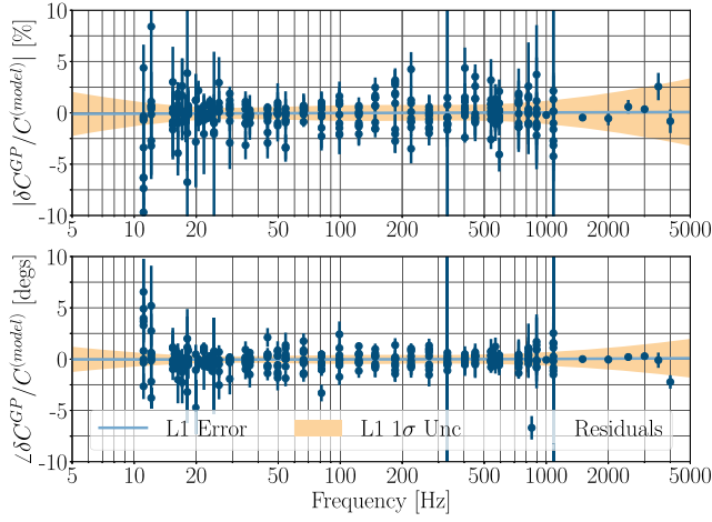
FIG. 7. Gaussian process regression of L1's sensing systematic error \delta C^{GP}(f) . The dark blue points are all the sensing measurement residuals, \delta C/C^{(\text{model})}(f, t, \vec{\lambda}_C) , taken over the entire observation run. This includes the residuals from the L1 reference measurement in the far right plots of Fig. 3. The light blue line is the mean function representing systematic error. The light orange envelope is the 1\sigma uncertainty on the systematic error.
