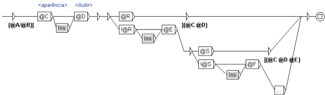
Fig. 1. Reference graph for the proverbs' database.
