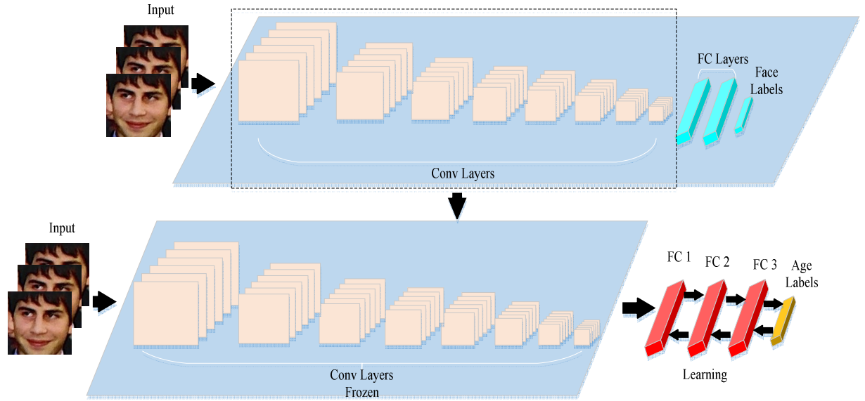
Figure 1. Fine-tuning domain specific pre-trained model for age classification.
