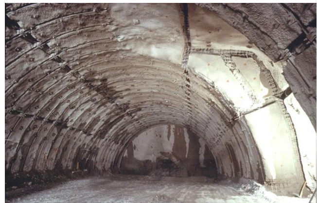
Figure 2. Support with open slots in the lining (Innatltunnel, Austria)
