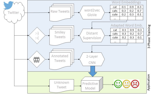
Figure 1: Training Phases Overview.
