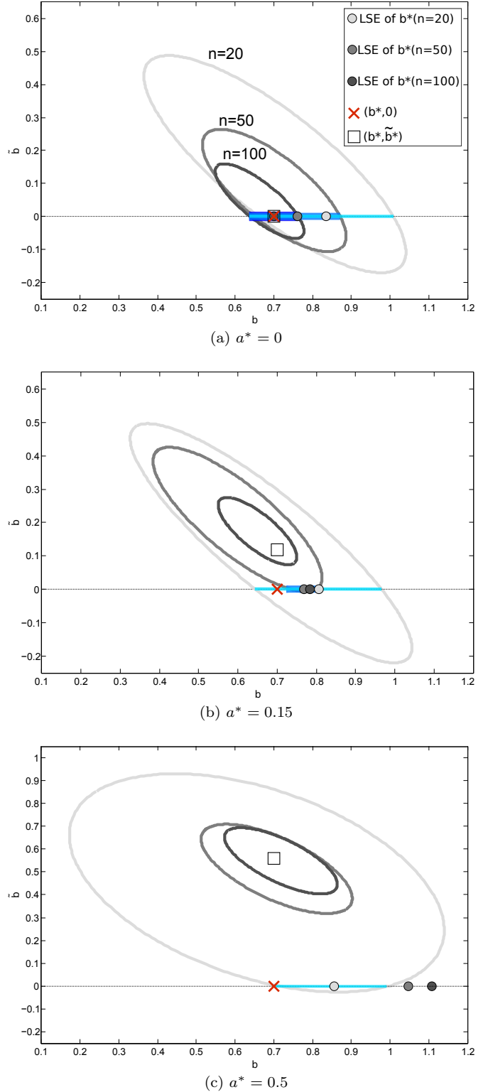
Fig. 1. In each of these pictures, the SPS ellipsoids \hat{\Theta}_n' in the 2-dimensional (augmented) space for n = 20 (light gray), n = 50 (gray), n = 100 (dark gray) are shown. The corresponding outer-approximation of the UD-SPS region, \hat{\Theta}_n^o , is obtained by intersecting the ellipsoid \hat{\Theta}_n' with the b -axis (horizontal line). The “true” parameter b^* is also represented in the 2-dimensional space as (b^*, 0) , together with the convergence point (b^*, \tilde{b}^*) of the SPS region in the 2-dimensional space. The circles on the b -axis denote the LS estimates of b^* , namely \hat{\theta}_{20} (light gray), \hat{\theta}_{50} (gray), and \hat{\theta}_{100} (dark gray).
