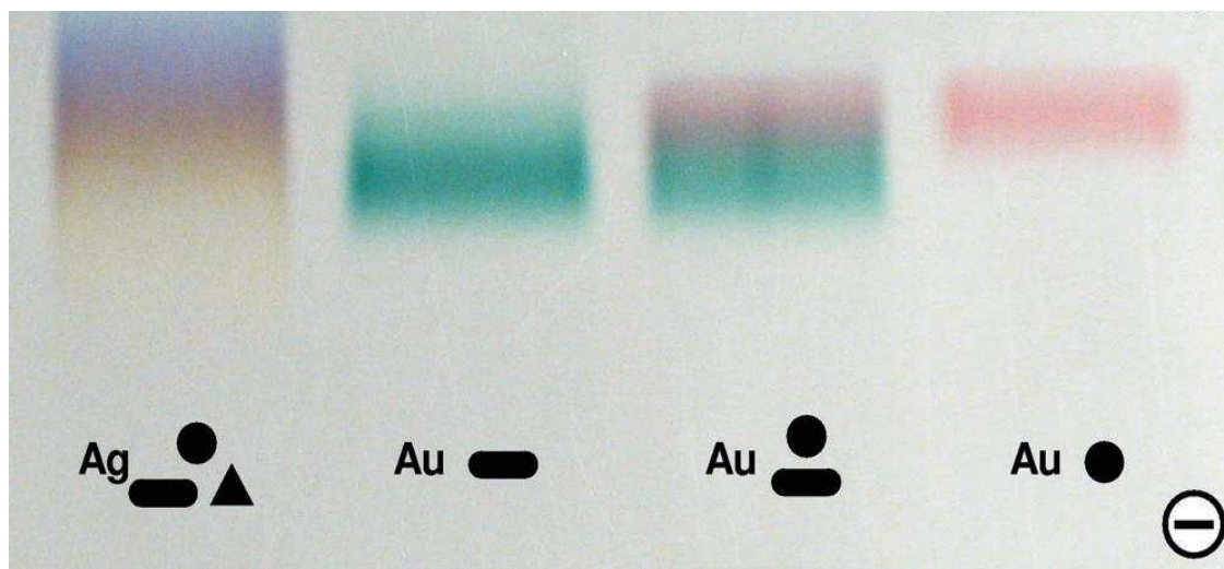
Figure 2-7 True colour photograph of a 0.2% agarose gel run for 30 min at 150 V (15 cm electrode spacing) at \text{pH} \approx 9 .
