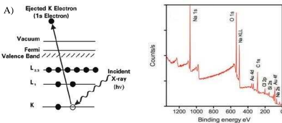
Figure 2-5 (A) The photoemission process in XPS surface analysis. The discs represent electrons and the bars represent energy levels within the material being analysed. The equation governing the process is KE = h\nu - BE , where KE is the photoelectron kinetic energy, h\nu is the exciting photon energy, and BE is the electron binding energy. Adapted from www.xpssimplified.com (B) XPS survey spectrum from citrate stabilized Au NPs showing various gold, sodium, oxygen peaks and a silicon peak. Reprinted with permission from (Sierra et al. 2016).
