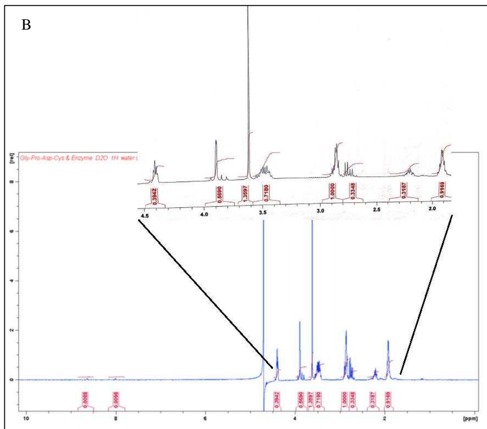
Figure 3-18 400 MHz ^1\text{H} NMR spectra of: (A) GPDC and (B) GPDC + DPP-IV.
