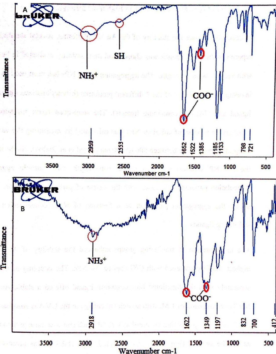
Figure 5-3 Infrared spectra of stabilized ligand GPDCALNNC (A) and GPDCALNNC capped Au NPs (B). Functional ligands inside red circles represent the shift in the band position and disappearance of thiol band suggesting a formation of thiolate-gold bond.
