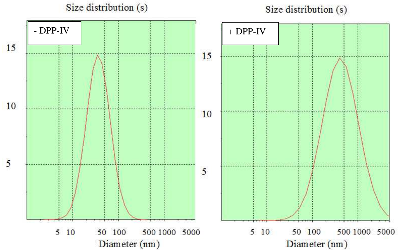
Figure 4-4 Hydrodynamic size distribution for modified Au NPs. before (left) and after (right) incubation with DPP-IV/ CD26.
