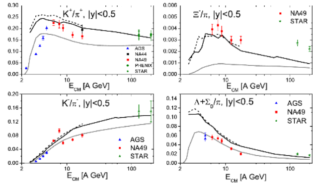
Fig. 2. Excitation function for kaon to pion ratios (left) and strange-baryon to pion ratios (right) for most central Au+Au/Pb+Pb collisions in the energy range \sqrt{s} = 2 - 200\text{A} GeV. The hybrid model calculations are the solid and dashed black line for two different freeze-out criteria. UrQMD 2.3 results and experimental data [2, 5, 26–29] are shown for comparison.
