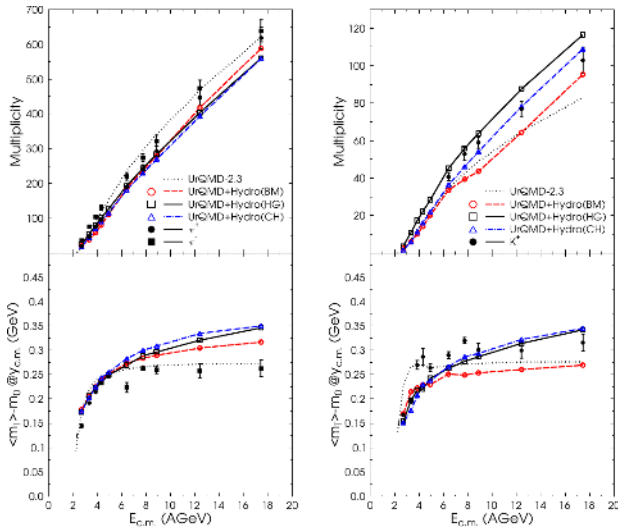
Fig. 1. Pion (left) and kaon (right) multiplicities (top) and mean transverse mass excitation function for central ( b < 3.4\text{fm} ) Au+Au/Pb+Pb collisions. The experimental data (full black symbols) are compared to hybrid model calculations with different equations of state (lines with symbols) and pure UrQMD 2.3 calculations (dashed line) [2, 5, 26–29]
