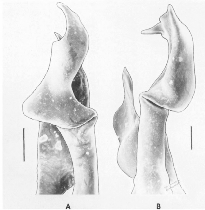
Fig. 1A: Gonopod (right) of Plicatodesmus turquino n. sp., ventral aspect. 1B. Gonopod (left) of Plicatodesmus baire n. sp., ventral aspect. (Scale line = 100 \mu )
