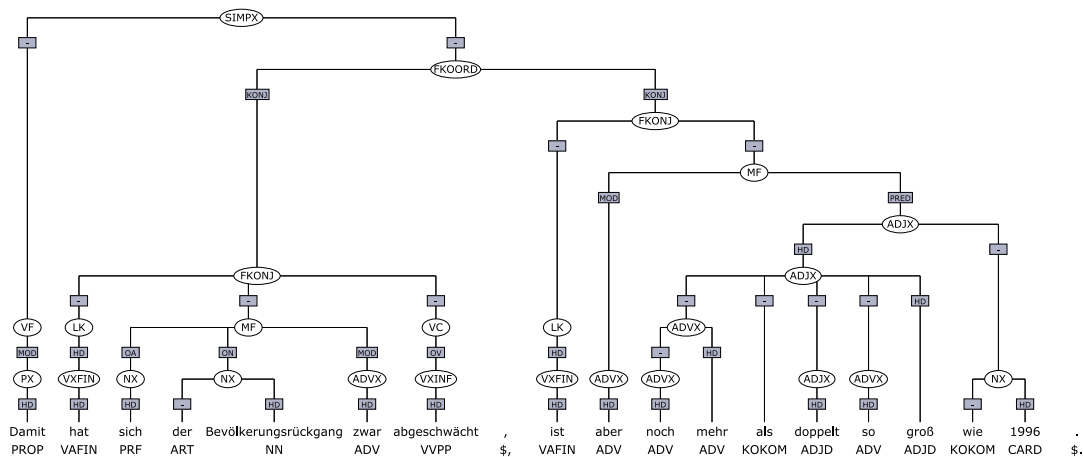
Figure 1: A tree with coordination.
