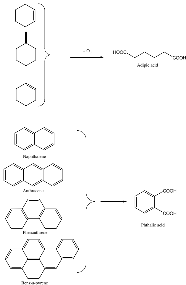
Fig. 3. Anthropogenic precursors of adipic and phthalic acid.
