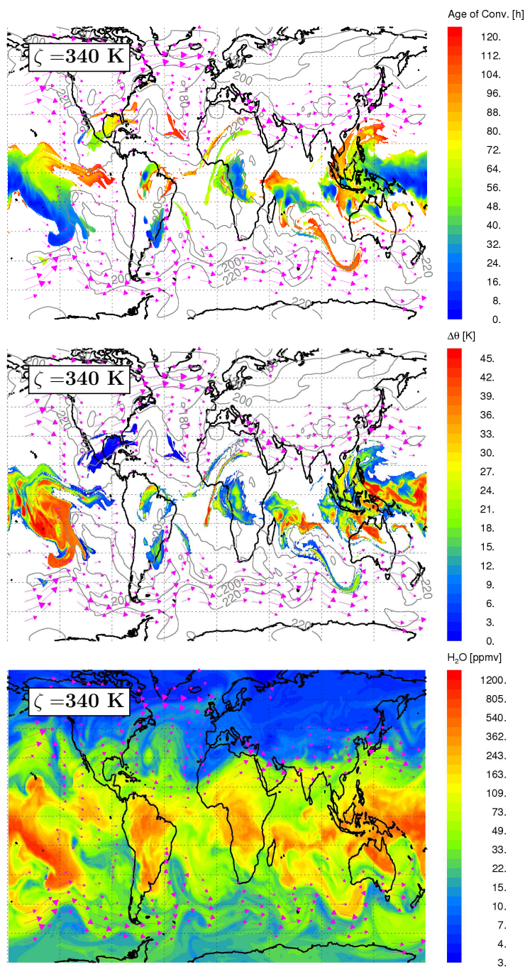
Fig. 3. Age of convection (top), \Delta\theta experienced along the trajectories (middle) and the ECMWF water vapor distribution at \zeta=340 \text{ K} (bottom). The age of convection is derived from the 5-day backward trajectories starting at this level on 8 February 2005, 12:00 UT, and is defined as the time lag between the initialization time and the time when the trajectory descended below p_c=300 \text{ hPa} . \Delta\theta denotes the increase of the potential temperature experienced by air parcels along these trajectories (positive values mean ascent with increasing time). Overlaid are wind vectors (pink) plotted for wind velocities higher than 20 \text{ m/s} and indicating the positions of STJs. The gray lines denote the pressure isolines.
