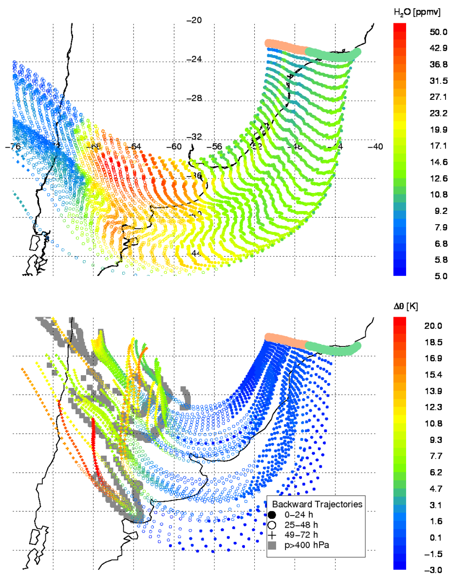
Fig. 11. 3-day backward trajectories starting on 8 February 2005 between 13:45 and 15:30 UT from the AB (beige) and BC (green) flight legs (top) or 25 K below these flight legs (bottom). Top: ECMWF \text{H}_2\text{O} interpolated along these trajectories. Bottom: \Delta\theta experienced by the air masses along the backward trajectories starting 25 K below the flight track. Positive (red) and negative (blue) values correspond to up- and downward motion of air with increasing time. The gray footprints are places where the trajectories cross the 400 hPa level. In the satellite pictures (GOES), fresh convective clouds could be found in the same region (see Fig. 12).
