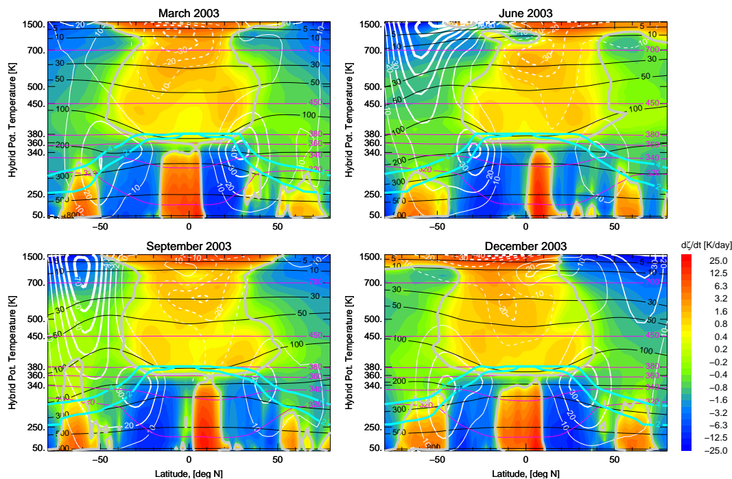
Fig. 4. Zonally and monthly averaged vertical velocities \zeta shown as a function of the entropy-weighted hybrid coordinate \theta (i.e. the entropy density along the vertical axis is constant). The gray contour defined by \zeta = 0 separates the ascent from descent regions. White contours (solid – westerlies, dashed – easterlies) describe the zonal wind. The isolines of pressure (black) and potential temperature (pink) are overlaid. The isolines |PV|=2 and 4 PVU together with the \theta = 380 K line (blue) approximate the position of the tropopause in the extratropics and in the tropics, respectively.
