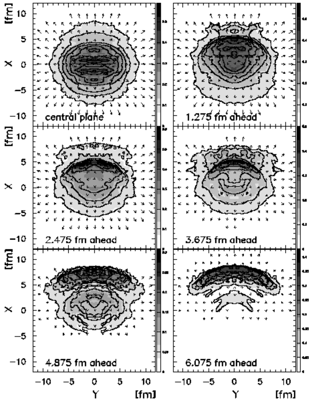
Figure 4: Contour plots of R in the tranverse x - y -plane at several values of z > 0 (forward hemisphere).
