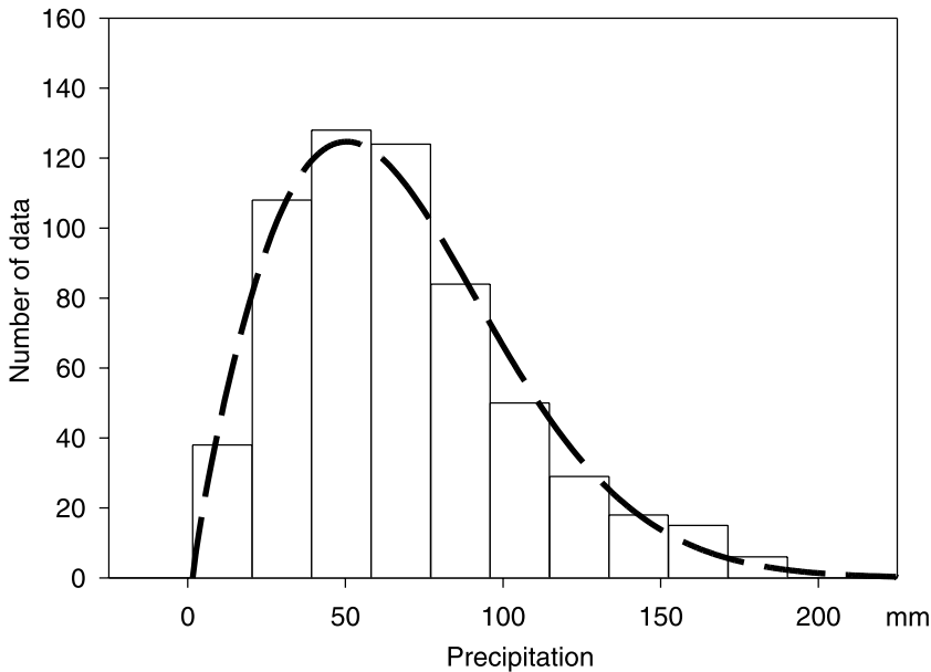
Fig. 3. Similar to Fig. 2, but second half of observation period (1946–1995)
