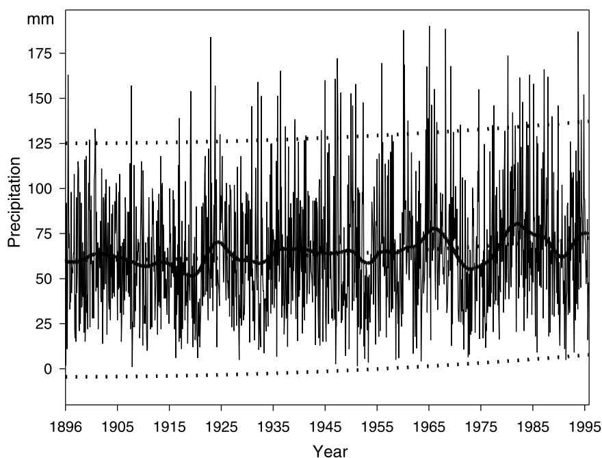
Fig. 1. Monthly total precipitation time series 1896–1995 Eppenrod (Central Germany, 50.4° N 8.0° E) including a progressive trend of order 2 detected by time series component analysis and related \pm 2\sigma boundaries (dashed lines, \sigma = standard deviation), furthermore 10 yr low-pass filtered data (heavy line) indicating a roughly 20 yr cyclical component, however, significant only within the recent three decades and irregular in earlier time
