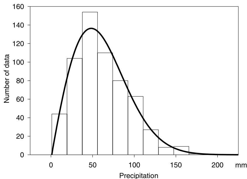
Fig. 2. Empirical frequency distribution of the time series plotted in Fig. 1, first half of observation period (1896–1945), columns, and fitting of a Weibull probability density function (heavy line)
