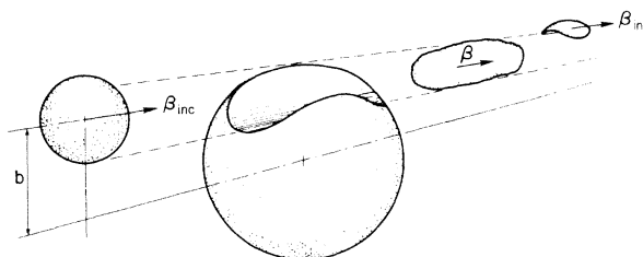
FIG. 1. A neon nucleus is incident on the uranium nucleus with a velocity \beta_{inc} in the laboratory frame and impact parameter b . The swept-out nucleons from the projectile and target are called the fireball, and their center of mass has the velocity \beta in the laboratory frame.
