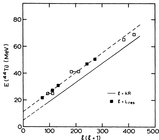
FIG. 7. Rotational band formed by the resonant angular momenta L of backward \alpha - ^{40}\text{Ca} scattering. The plot gives L(L+1) versus the excitation energy in the compound system ^{44}\text{Ti} . Ambiguous L assignments are indicated. The band-head energy is about 10 MeV. The full line represents l_0(l_0+1) for the grazing angular momenta l_0 .
