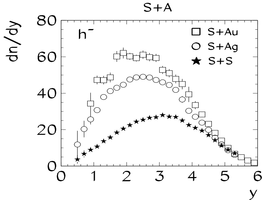
Figure 23. Rapidity distributions of negatively charged hadrons produced in central S-nucleus collisions.
