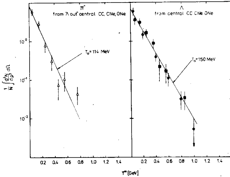
Fig.6. The spectrum of the kinetic energy T^* calculated in the N-N c.m. system for " \Lambda out" pions and \Lambda hyperons produced in central collisions of nuclei ( A_P = A_T ). T_0 - the temperature parameter.
