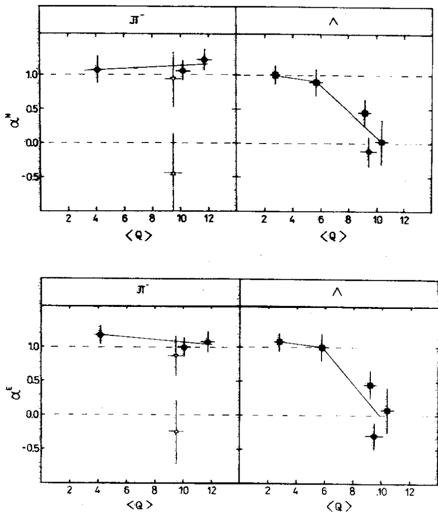
Fig.3,4. The \alpha^N (fig.3) and \alpha^E (fig.4) values (for definition see text) versus \langle Q \rangle , the average number of participant protons for \pi^- mesons and \Lambda hyperons. The dashed lines show the values corresponding to the flat \cos\theta^* distribution and to the \cos\theta^* distribution observed in inelastic HeLi collisions. Circles - data obtained in the streamer chamber experiment; squares - data obtained in the propane bubble chamber experiment; triangles - data corresponding to " \Lambda_{in} " ( \nabla ) " \Lambda_{out} " ( \Delta ) pions. The solid lines are drawn to guide the eye only.
