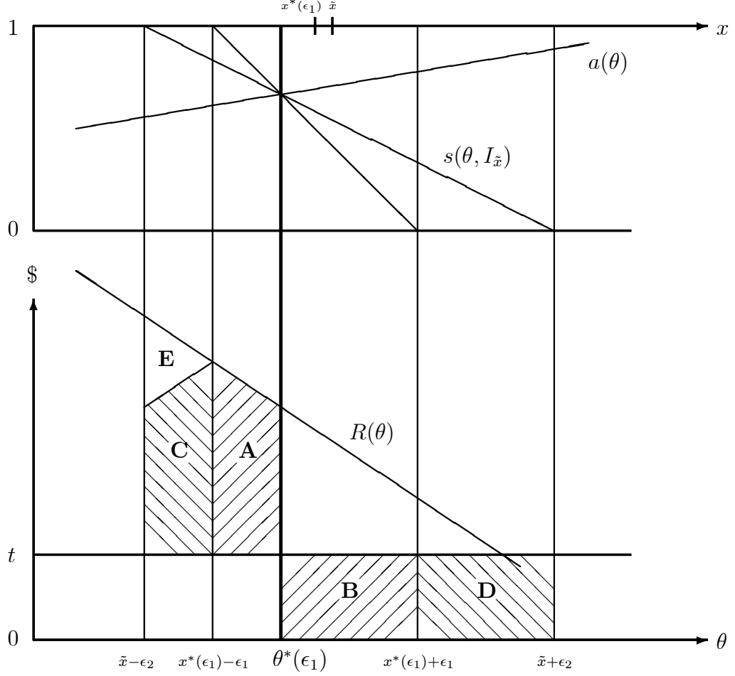
Figure 3 Areas A and B are of equal size, so that x^*(\epsilon_1) and \theta^*(\epsilon_1) are the equilibrium switching point and threshold for signals distributed uniformly in an \epsilon_1 surrounding of the true state. If dispersion is increased to \epsilon_2 and strategies are adjusted to I_{\tilde{x}} , such that the threshold remains \theta^*(\epsilon_1) , then expected gains are given by A + C + E and exceed expected losses B + D by the triangular area E . Note that for \epsilon_2 = 2\epsilon_1 , area C = A and D = B .
