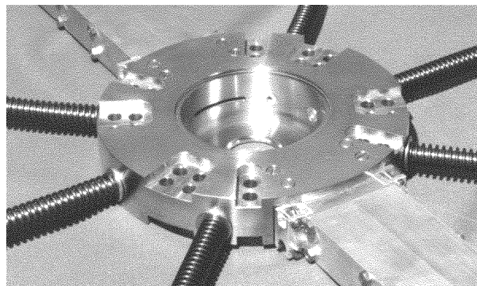
Fig. 1: The wall slotted damping cell.
