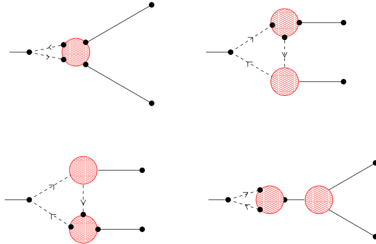
FIG. 5: Connected part of 4-point GF \overline{CC}Q_1Q_2 , corresponding to Eq. (B9).
