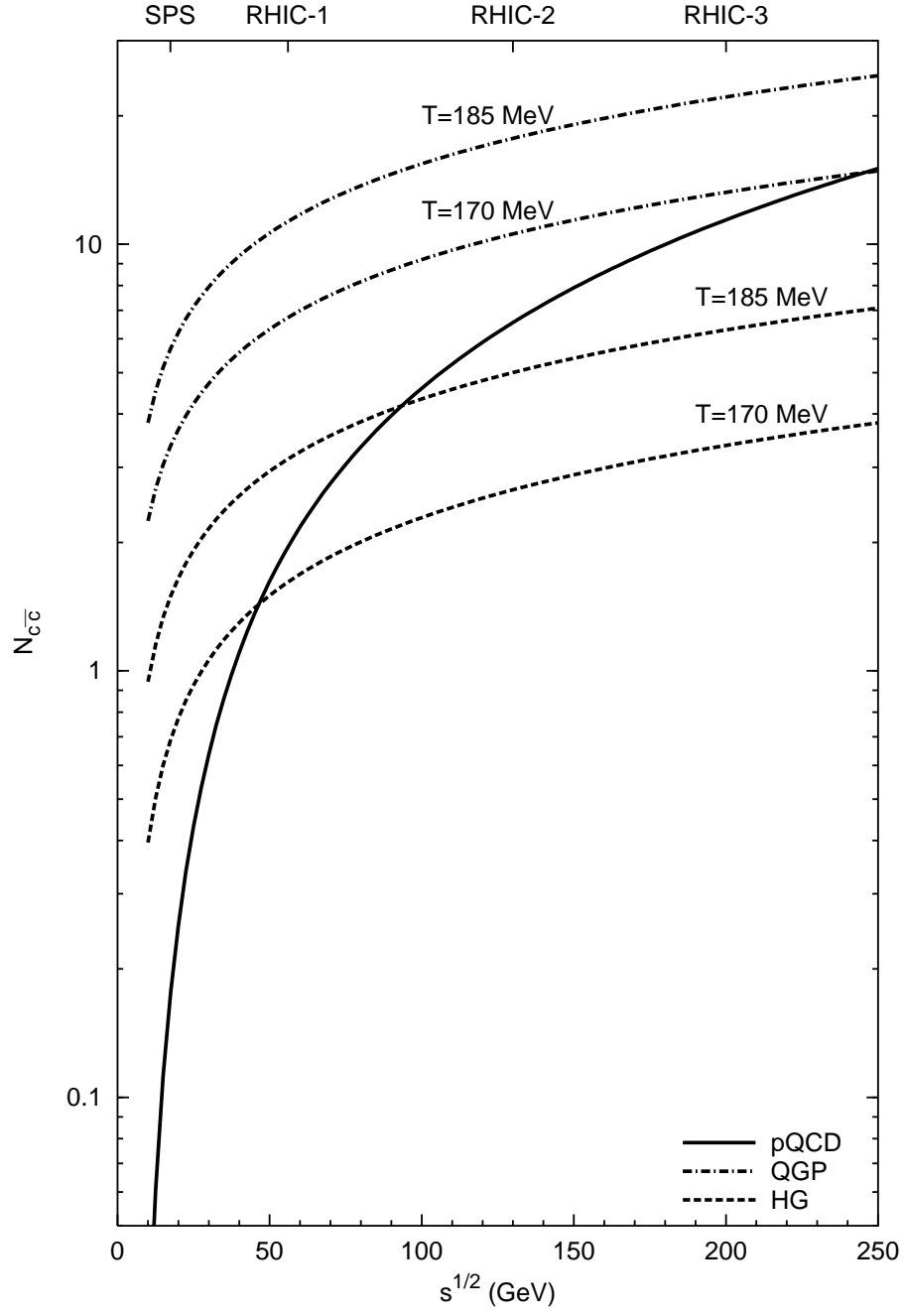
FIG. 1. The dependence of the average number of c\bar{c} pairs per Au+Au central collision on the center-of-mass energy of the nucleon pair. The calculations are done in the framework of three different models: perturbative QCD (pQCD), equilibrium quark-gluon plasma (QGP), equilibrium hadron gas (HG). The QGP and HG results are shown for two different temperatures: T = 170 MeV and T = 185 MeV.
