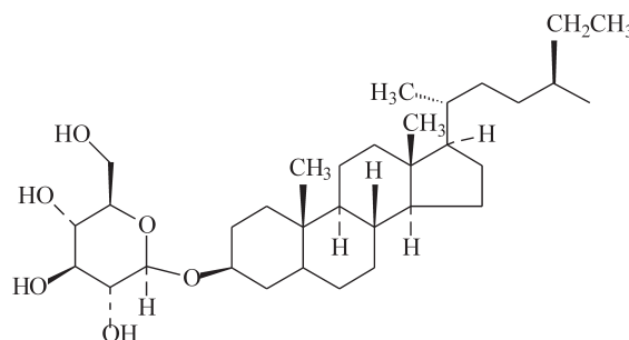
Fig. 2. \beta -Sitosterol glucoside (BSSG).
