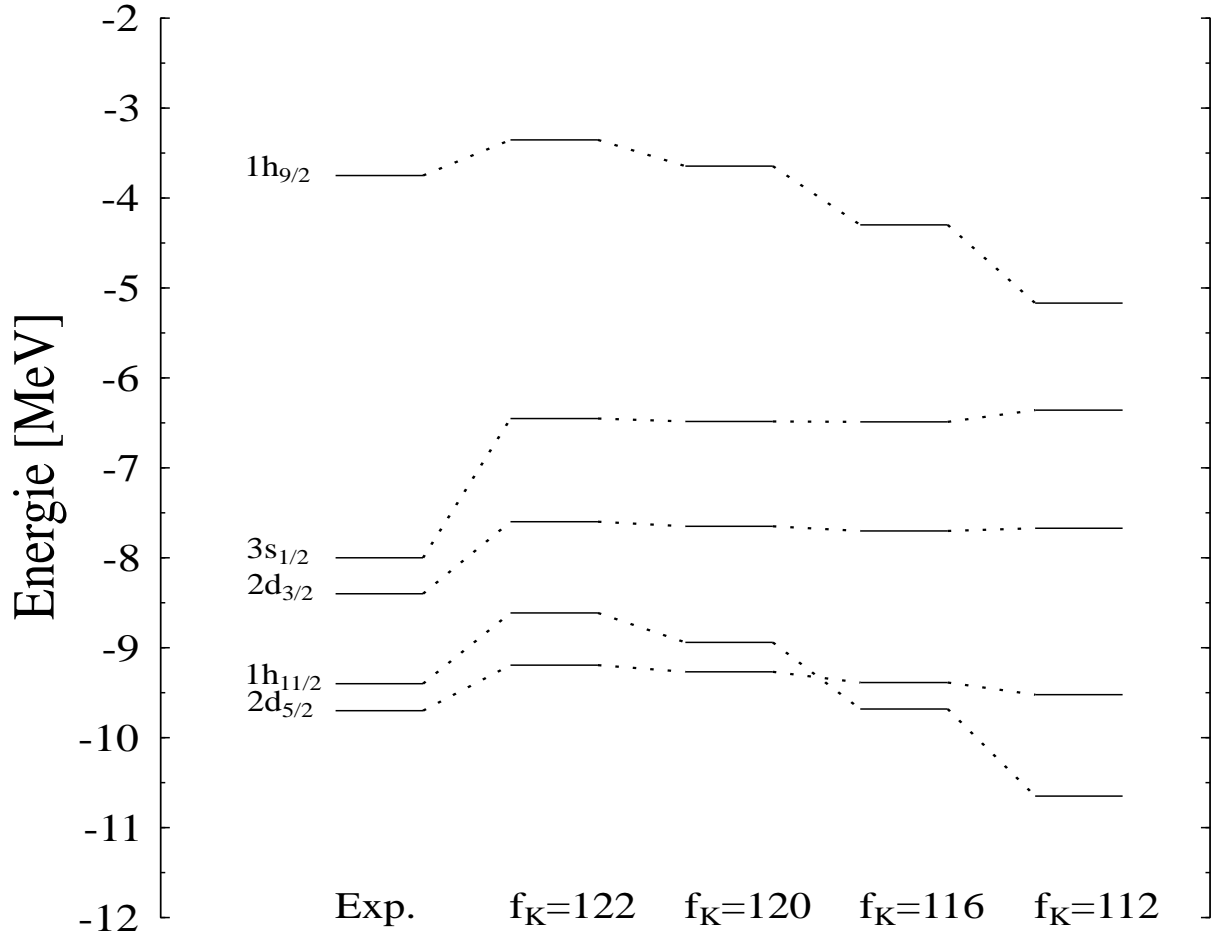
FIG. 2. Single particle energy levels for protons in Pb^{208} for parameter sets with different values of the kaon decay constant f_k (in MeV ). The smaller the decay constant is chosen, the more the gap between the levels 1h_{\frac{9}{2}} and 3s_{\frac{1}{2}} decreases. The parameter sets were obtained by just varying f_k in C_1 .
