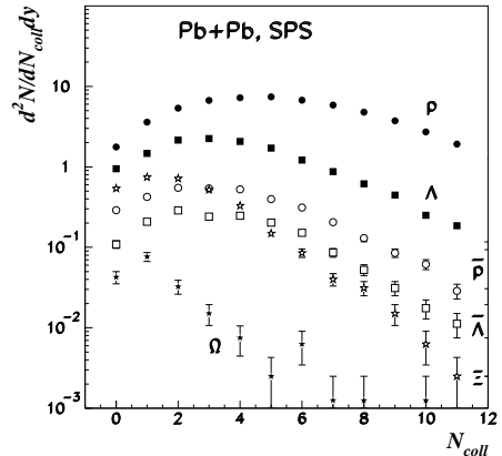
FIG. 2. Distribution of the number of interactions that the final-state particles suffer after being hadronized.
