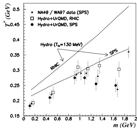
FIG. 3. Inverse slopes of the m_T -spectra of \pi , K , p , \Lambda + \Sigma^0 , \Xi^0 + \Xi^- , and \Omega^- at y_{c.m.} = 0 , m_T - m_i < 1 GeV.
