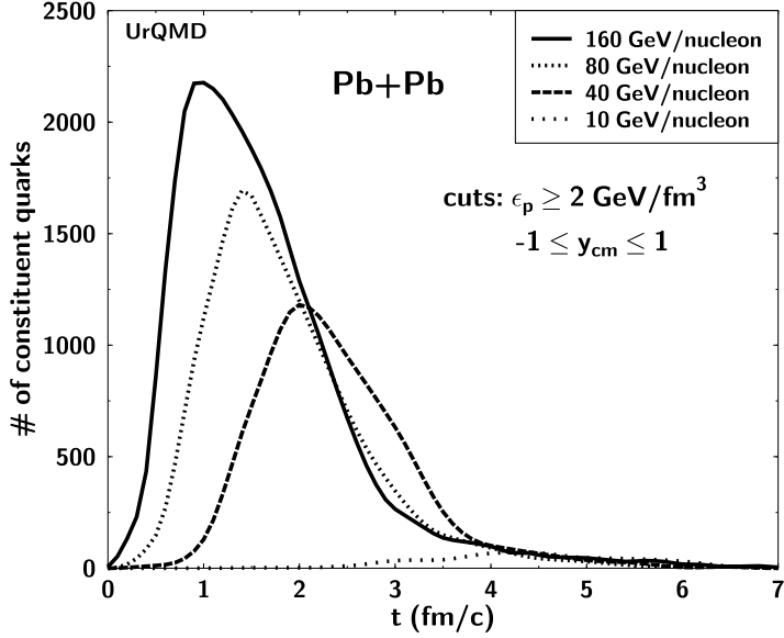
FIG. 3. Multiplicity of “constituent quarks” propagating through a “partonic” energy density of \epsilon_Q \geq 2 \text{ GeV/fm}^3 . The number of “constituent quarks” is obtained by summing over all partonic constituents, weighting the developing baryons by a factor of 3 and mesons-to-be by a factor of 2, respectively. At 160 GeV > 1000 “constituent quarks” are present over a time scale of \Delta t \approx 2 \text{ fm/c} .
