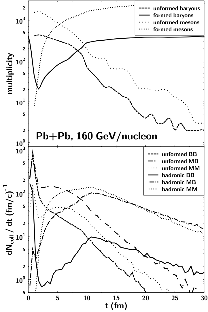
FIG. 2. Top: Time evolution of the multiplicity of hadrons and partonic constituents, divided into baryonic and mesonic contributions. Bottom: Collision rates for baryon-baryon (BB) and meson-meson (MM) collisions. The rates have been decomposed into interactions involving formed hadrons and those involving partonic constituents.
