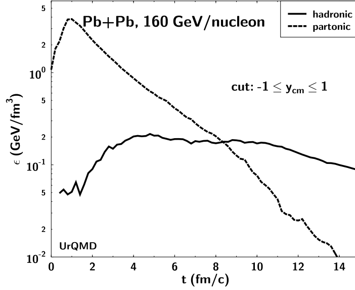
FIG. 1. Time evolution of the energy density \epsilon in central Pb+Pb reactions at 160 GeV/nucleon. \epsilon has been decomposed into “partonic” and “hadronic” contributions and only particles around mid-rapidity have been taken into account. The early and intermediate reaction stages are dominated by the “partonic” contribution.
