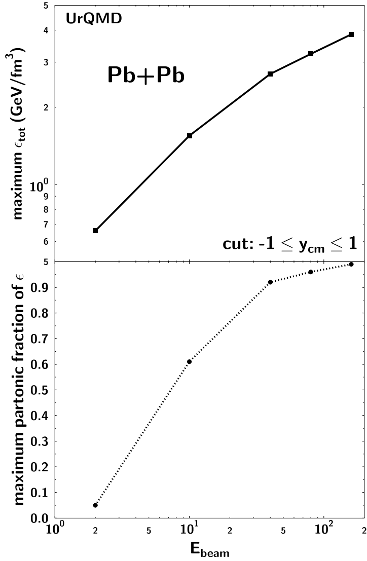
FIG. 4. Top: excitation function of the maximum total energy density mid-rapidity hadrons experience. Bottom: excitation function of the maximum “partonic” fraction of energy density. Already at a beam energy of 40 GeV/nucleon more than 90% of the energy density is contained in partonic degrees of freedom at one time during the collision.
