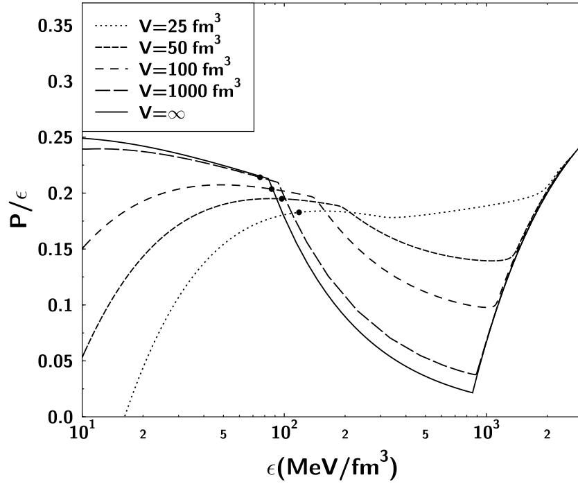
FIG. 6. Pressure P divided by the energy density \epsilon vs. the the energy density for systems of different sizes. The bag constant is B^{1/4} = 200 MeV. The color singlet constraint is taken into account for the QGP equation of state.
