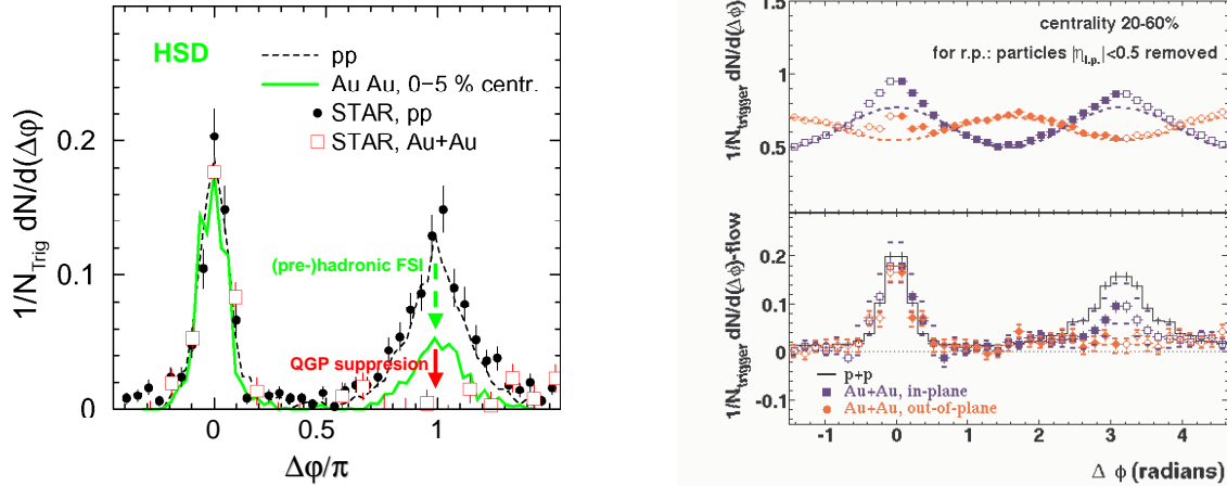
Figure 10. Left: STAR data on near-side and away-side jet correlations compared to the HSD model for p+p and central Au+Au collisions at midrapidity for p_T^{Trig} = 4 \dots 6 \text{ GeV}/c and p_T = 2 \text{ GeV}/c \dots p_T^{Trig} [28, 29]. Right: High p_T correlations: in-plane vs. out-of-plane correlations of the probe (jet+secondary jet fragments) with the bulk ( v_2 of the plasma at p_T > 2 \text{ GeV}/c ), prove the existence of the initial plasma state (STAR-collaboration, preliminary).
