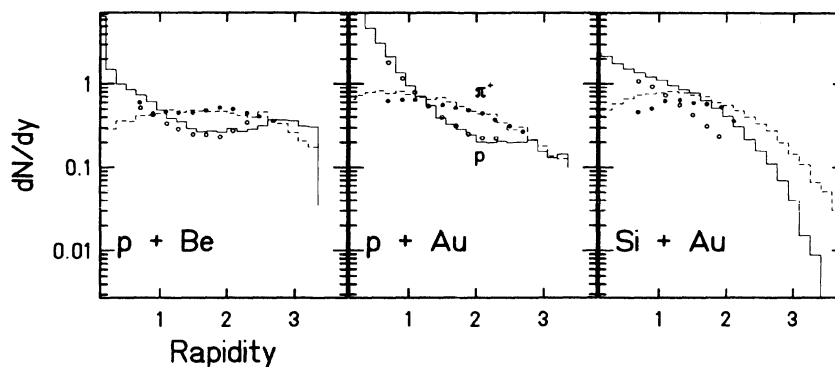
FIG. 3. Calculated and experimental meson rapidity distributions for minimum-bias p+\text{Be} (left), p+\text{Au} (middle), and central Si+Au (right) reactions at a projectile energy of 14.5A GeV. The histograms represent the RQMD results: protons (solid lines) and \pi^+ (dashed lines). The experimental data are shown for protons as open circles and for \pi^+ as solid circles. The Si+Au distributions are divided by 28.
