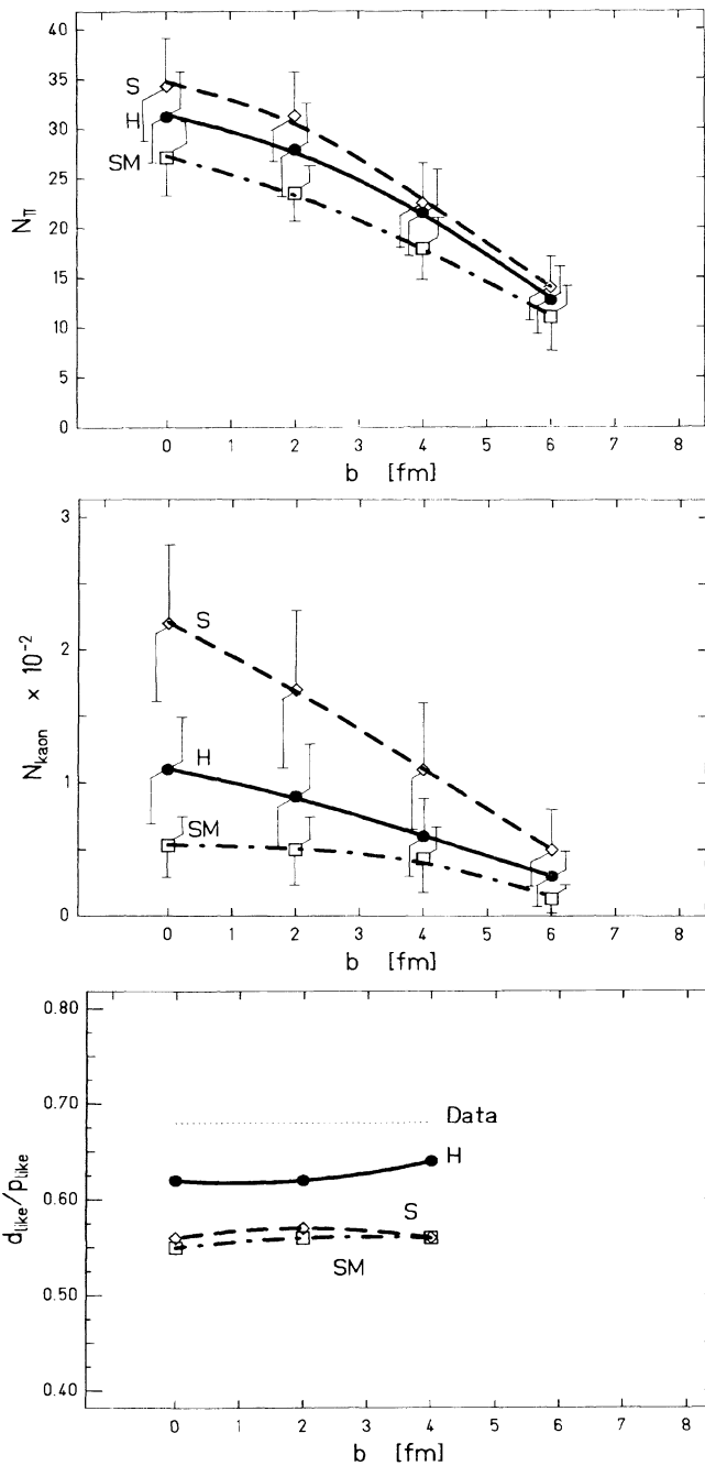
FIG. 2. The impact-parameter dependence of the kaon and pion yields and the deuteronlike to protonlike ratio R is shown for the system La(0.8 GeV/nucleon)+La for the S, SM, and H interactions. Note that the MDI lead to a suppression of the pion and kaon yields which by far exceeds the suppression due to a hard local potential. The d/p ratios, on the other hand, are insensitive to the momentum-dependent interactions.
