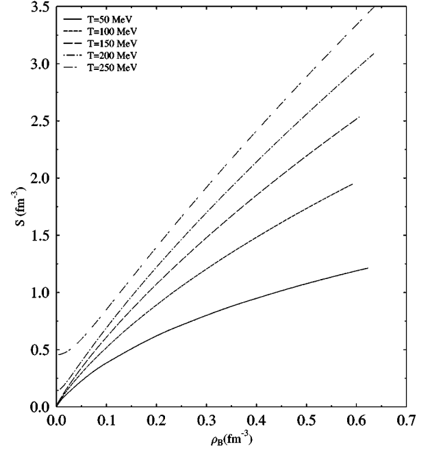
FIG. 3. The entropy density vs the density for various temperatures.
