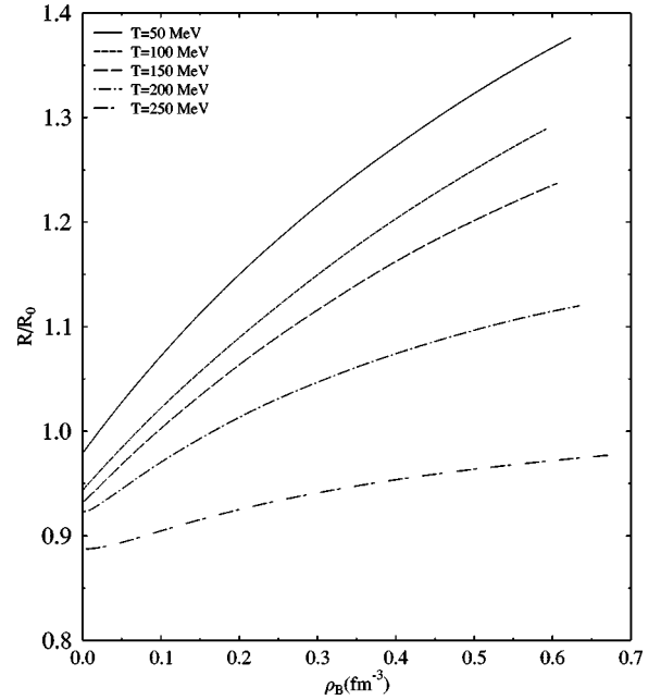
FIG. 6. The bag radius as a function of density at various temperatures; the nucleon bag size shrinks with temperature.
