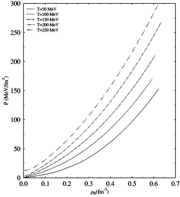
FIG. 1. The pressure for nuclear matter as a function of the baryon density \rho_B for various values of temperature showing an increase with temperature.
