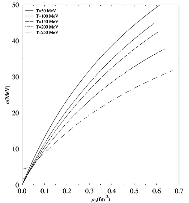
FIG. 4. The mean field \sigma as a function of density for different temperatures.
