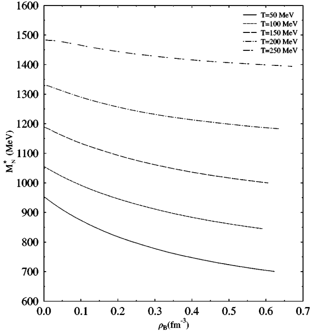
FIG. 2. The effective nucleon mass for nuclear matter as a function of the baryon density \rho_B for different values of the temperature, which is seen to rise monotonically with temperature.
