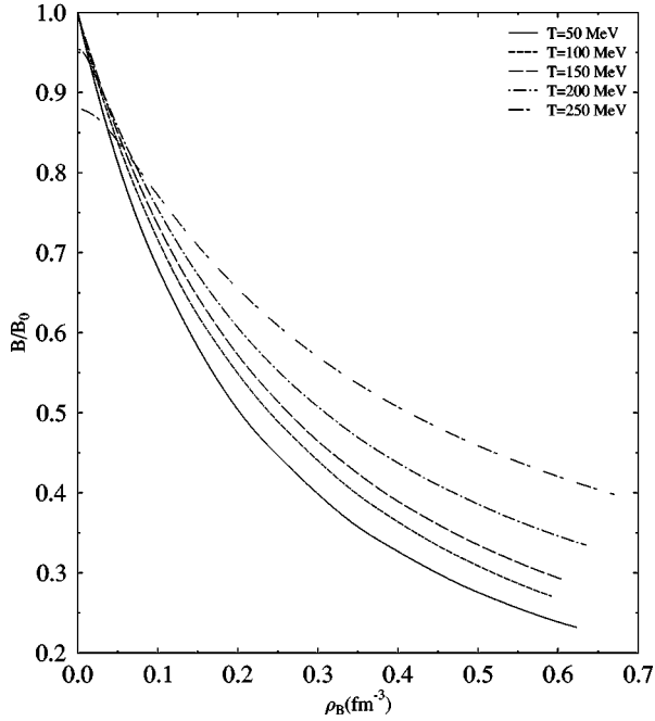
FIG. 5. The bag constant vs the density for different temperatures. It grows with temperature, except for very low densities and temperatures at and above 200 MeV.
