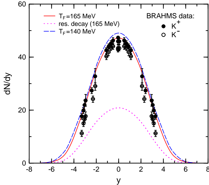
Fig. 2. Same as Fig. 1, but for K^+ rapidity distributions.
