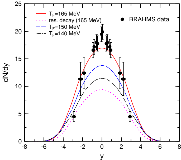
Fig. 3. Same as Fig. 1, but for antiproton rapidity distributions. All results are obtained assuming \mu_F = 0 . Experimental data are taken from Ref. [26].
