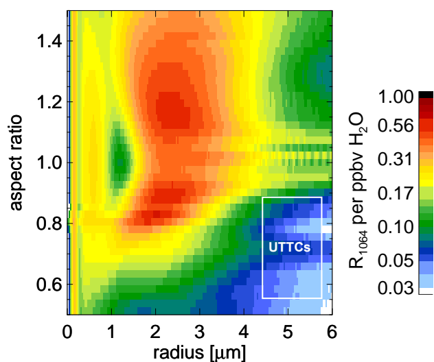
Fig. 8. Aerosol lidar backscattering ratio of 1 ppbv \text{H}_2\text{O} condensed as ice particles with radius and asphericity as indicated on the axes (aspect ratio defined as ratio between the axes perpendicular and parallel to the rotational symmetry). The aerosol backscatter is calculated by using the T-matrix method (Mishchenko, 1991) assuming that the particles are spheroids. The backscattering ratio can be scaled to other ice water content by just multiplying the scale shown in the right hand side by the amount of the actual ice water content in ppbv. The radius given here is the mode radius (equivalent sphere) of a lognormal size distribution with mode width \sigma = 1.20 . The white box in the lower right corner indicates the region of interest for UTTCs.
