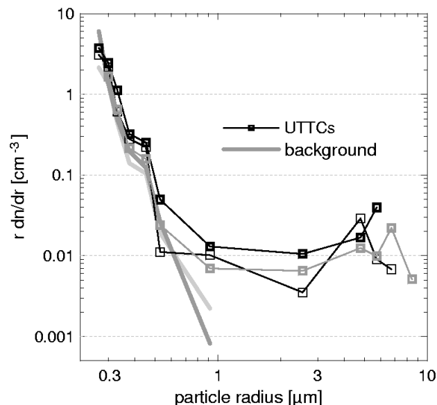
Fig. 7. Particle size distributions as function of (equivalent sphere) radius r measured by the FSSP-300 on board of Geophysica on 24 February 1999. Open squares: measurements inside UTTCs from several cloud encounters (see Fig. 4 and Fig. 3 between points D and F). Lines without symbol: background aerosols in the immediate vicinity below or above UTTCs.
